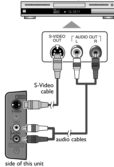
BD/DVD recorder, camcorder and VCR with the S-Video output jack
